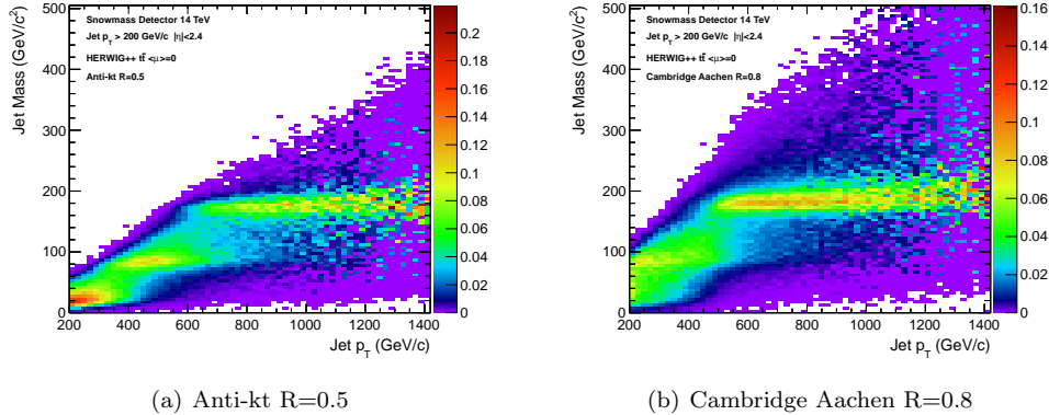
Figure 1-9. Jet mass vs jet transverse momenta in the DELPHES fast simulation for pp collisions at 14 TeV for different jet algorithms. The jet transverse spectrum has been reweighed to be flat.
