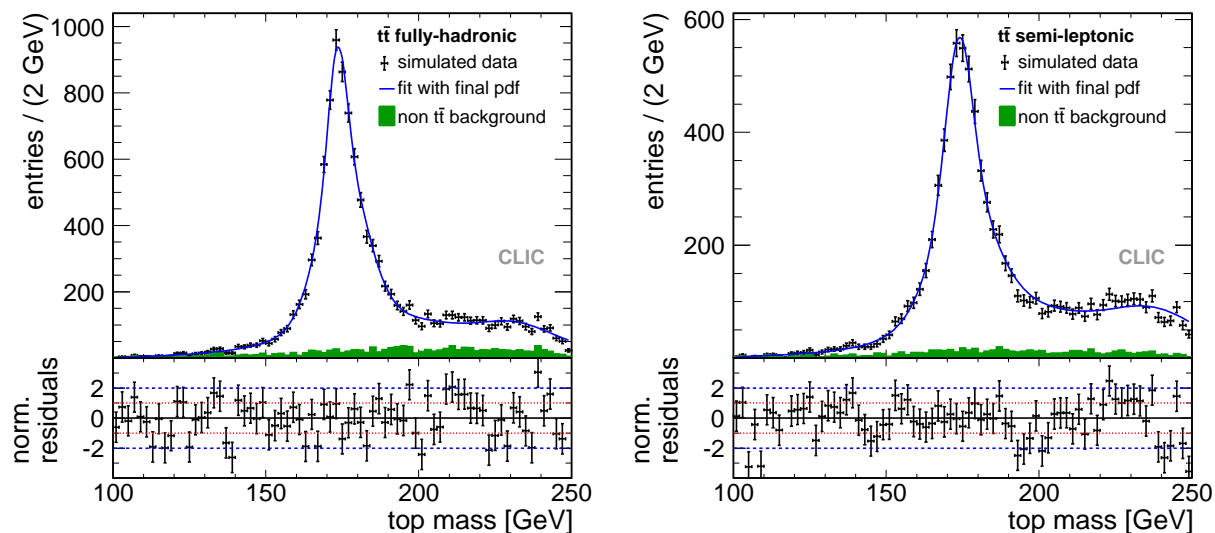
Figure 1-11. Distribution of reconstructed top mass for events classified as fully-hadronic (left) and semi-leptonic (right). The data points include signal and background for an integrated luminosity of 100\text{ fb}^{-1} . The pure background contribution contained in the global distribution is shown by the green solid histogram. The top mass is determined with an unbinned likelihood fit of this distribution, which is shown by the solid line.
