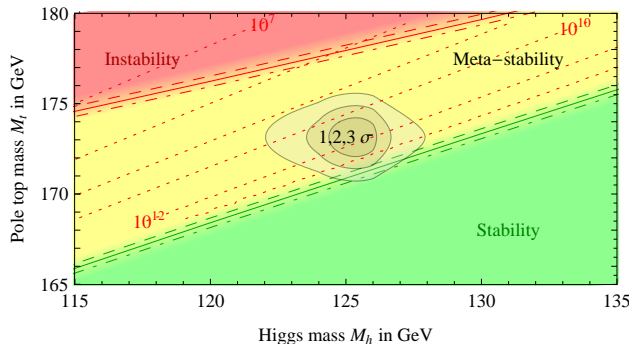
Figure 1-7. Regions of metastability and instability of the Higgs potential in the SM, as the top quark and Higgs boson masses are varied, from [40].
