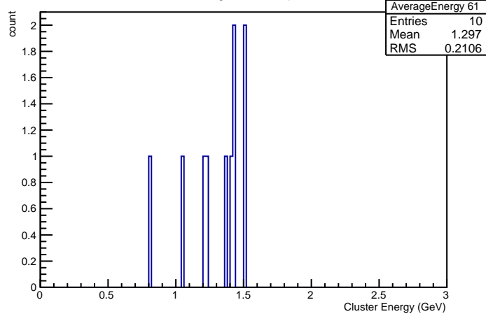
Cluster Energies in Crystal nr 61
