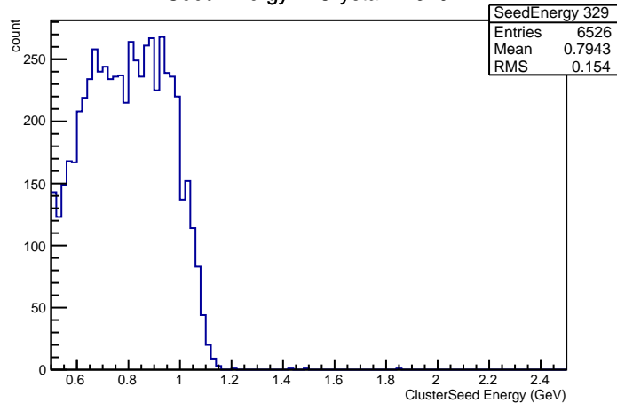
Seed Energy in Crystal nr 329
