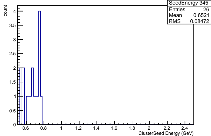
Seed Energy in Crystal nr 345
