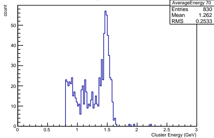
Cluster Energies in Crystal nr 70
