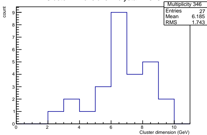
Cluster Dimensions in crystal nr 346
