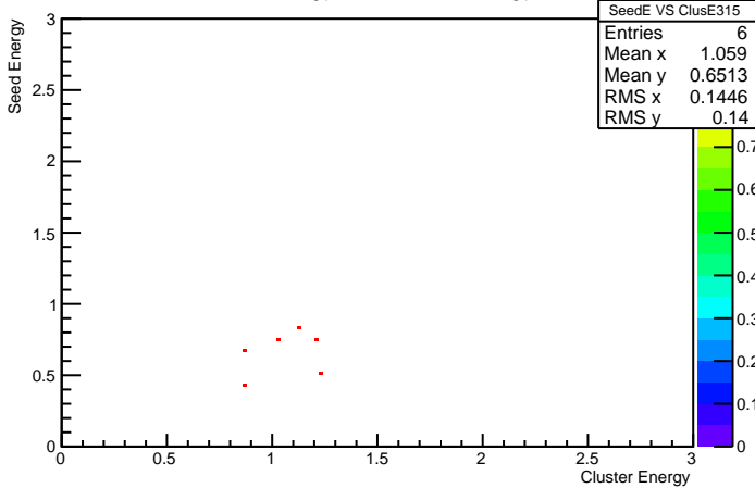
Cluster Energy VS Seed Energy 315
