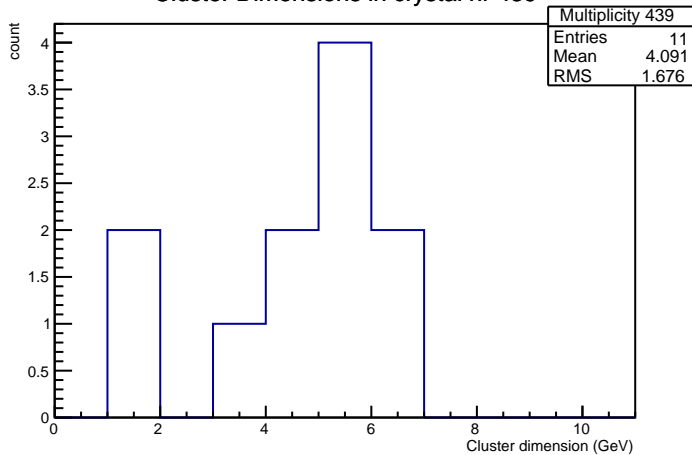
Cluster Dimensions in crystal nr 439
