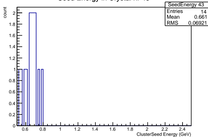
Seed Energy in Crystal nr 43
