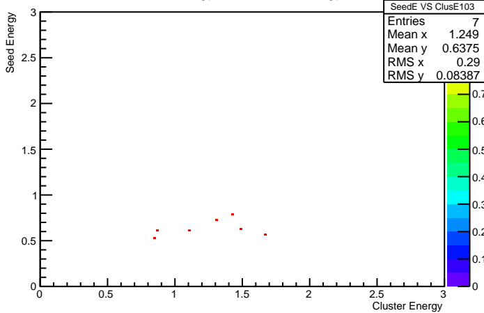
Cluster Energy VS Seed Energy 103
