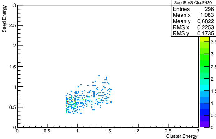
Cluster Energy VS Seed Energy 430
