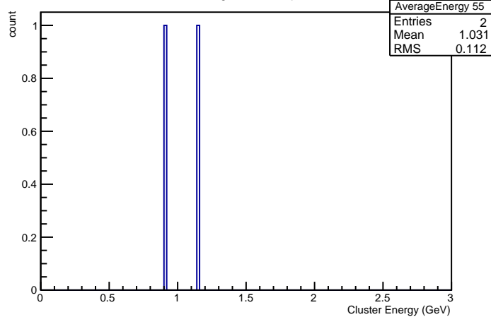
Cluster Energies in Crystal nr 55
