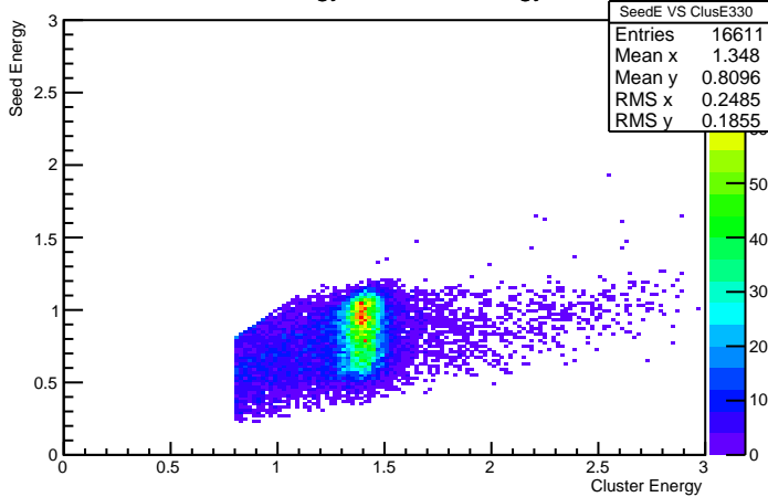
Cluster Energy VS Seed Energy 330
