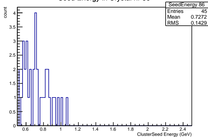
Seed Energy in Crystal nr 86
