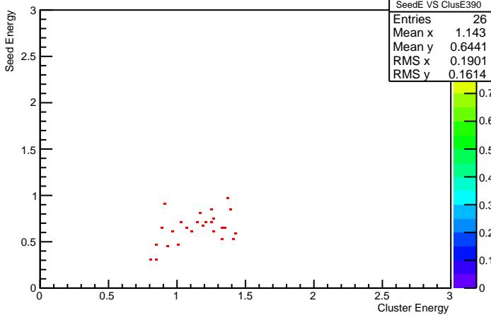
Cluster Energy VS Seed Energy 390
