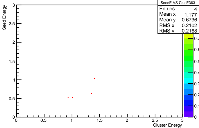
Cluster Energy VS Seed Energy 363
