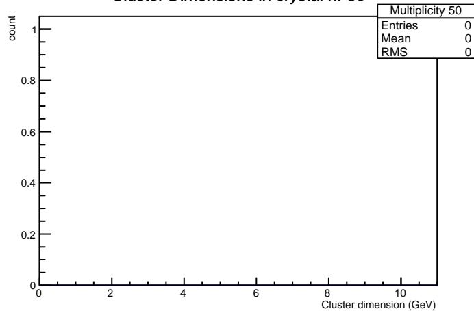
Cluster Dimensions in crystal nr 50
