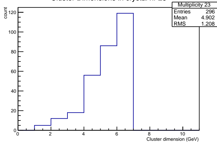
Cluster Dimensions in crystal nr 23
