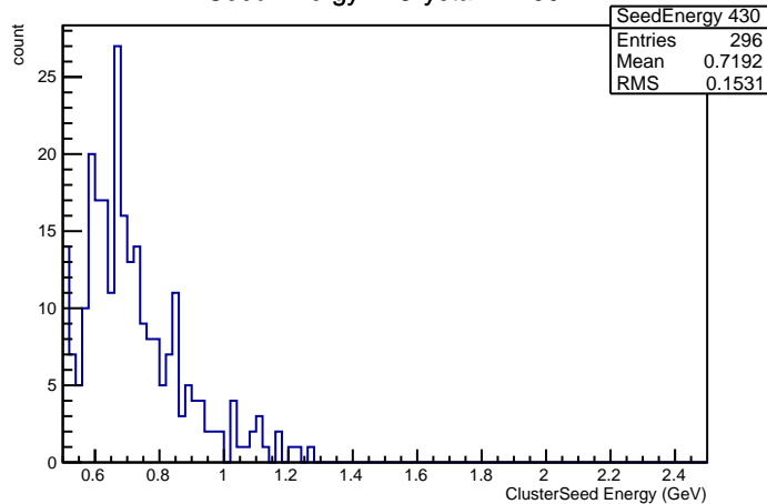
Seed Energy in Crystal nr 430
