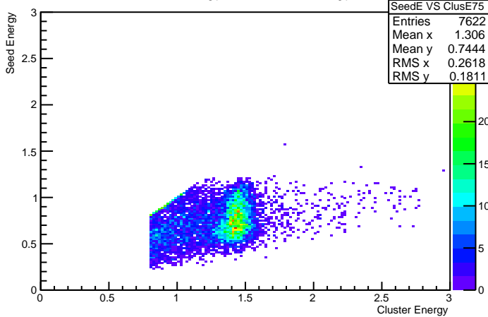
Cluster Energy VS Seed Energy 75
