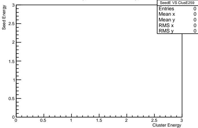
Cluster Energy VS Seed Energy 259
