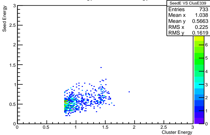
Cluster Energy VS Seed Energy 339
