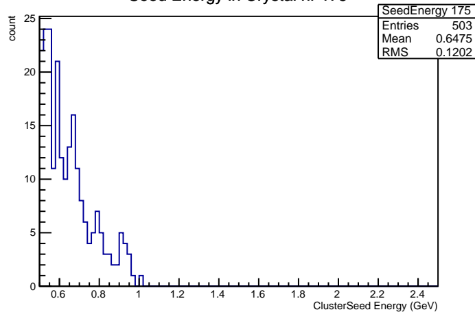
Seed Energy in Crystal nr 175
