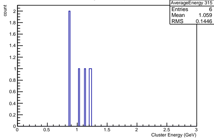
Cluster Energies in Crystal nr 315
