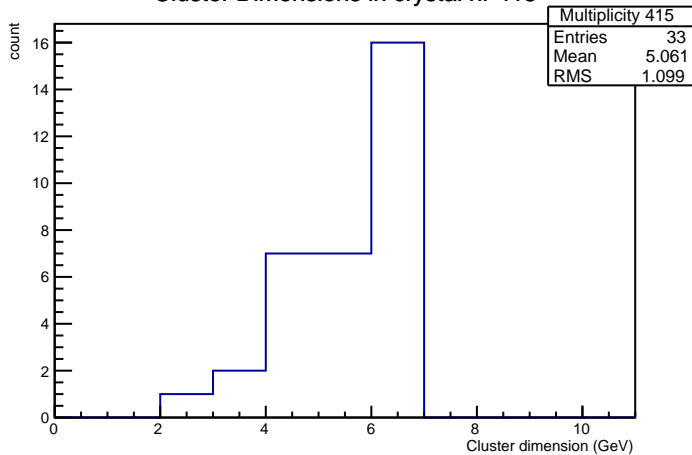
Cluster Dimensions in crystal nr 415
