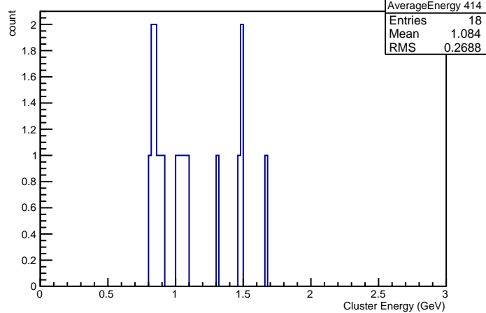
Cluster Energies in Crystal nr 414
