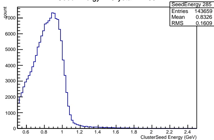
Seed Energy in Crystal nr 285
