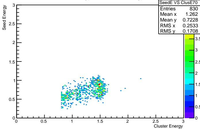
Cluster Energy VS Seed Energy 70
