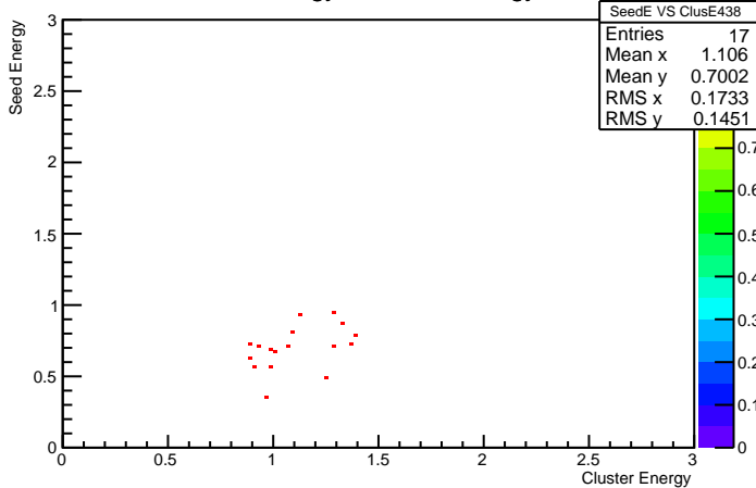
Cluster Energy VS Seed Energy 438
