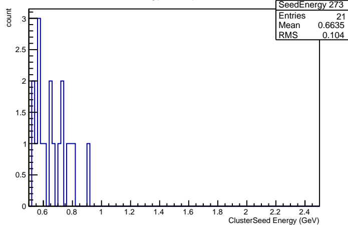
Seed Energy in Crystal nr 273
