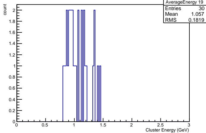
Cluster Energies in Crystal nr 19
