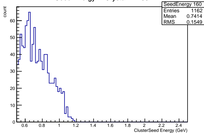
Seed Energy in Crystal nr 160
