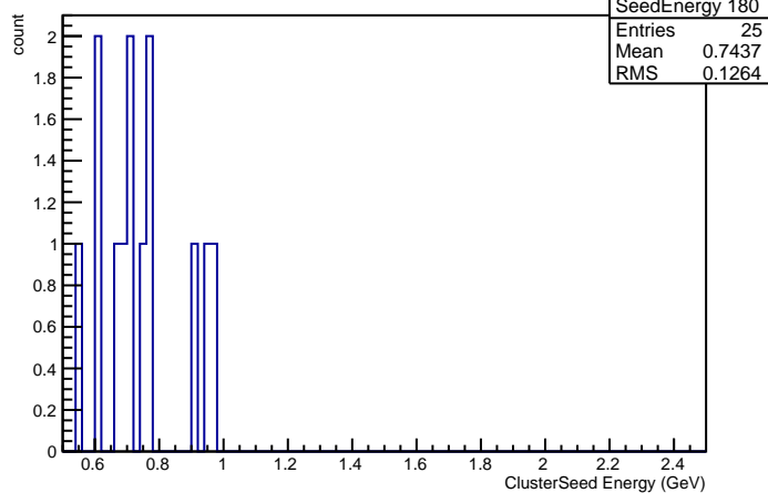
Seed Energy in Crystal nr 180
