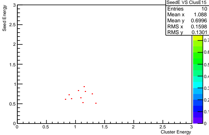
Cluster Energy VS Seed Energy 15
