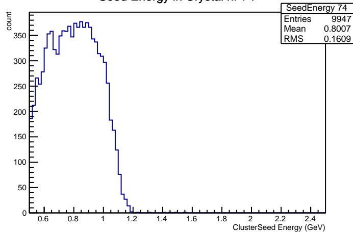
Seed Energy in Crystal nr 74
