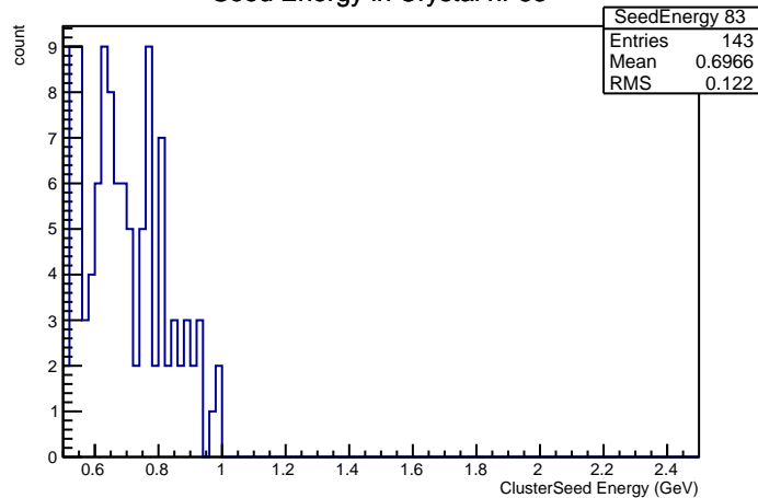
Seed Energy in Crystal nr 83
