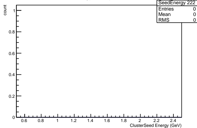
Seed Energy in Crystal nr 222
