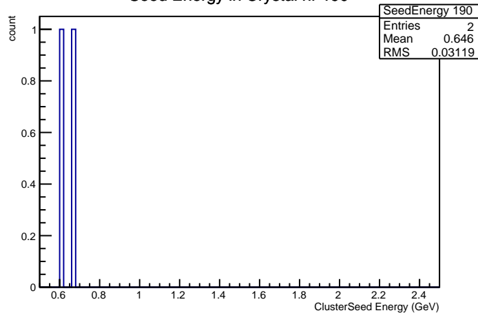
Seed Energy in Crystal nr 190
