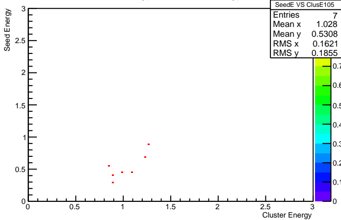
Cluster Energy VS Seed Energy 105
