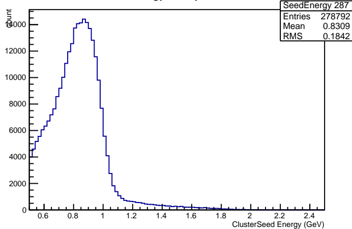
Seed Energy in Crystal nr 287
