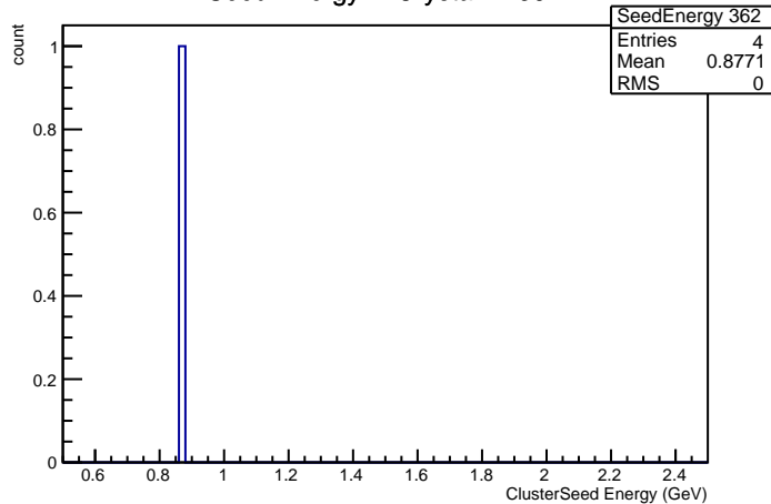
Seed Energy in Crystal nr 362
