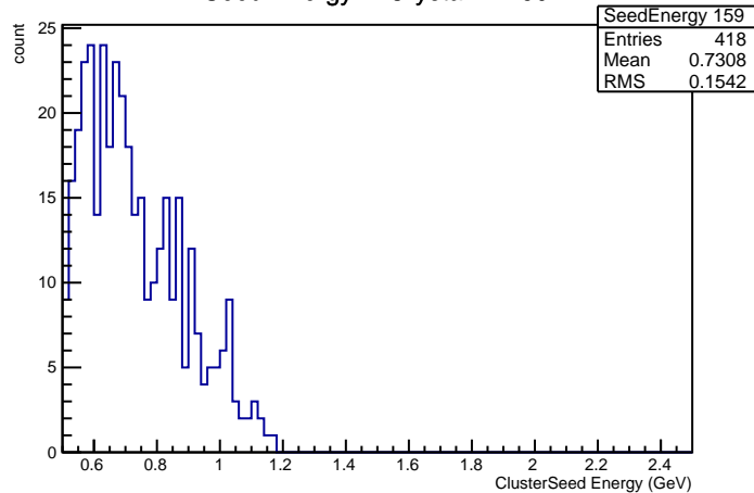
Seed Energy in Crystal nr 159
