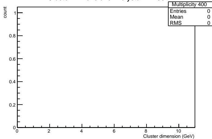
Cluster Dimensions in crystal nr 400
