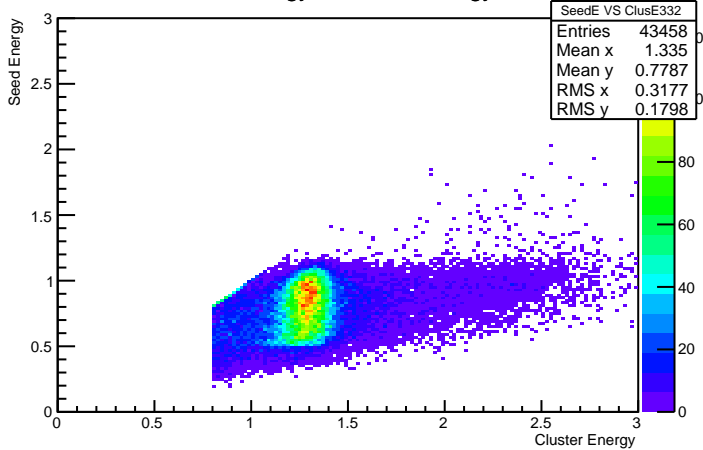
Cluster Energy VS Seed Energy 332
