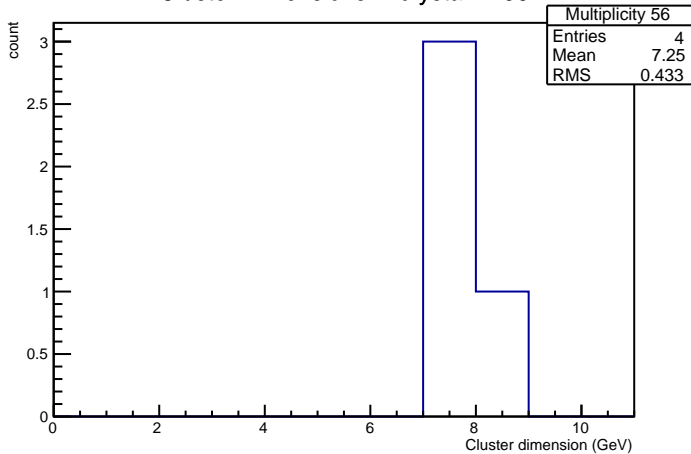
Cluster Dimensions in crystal nr 56
