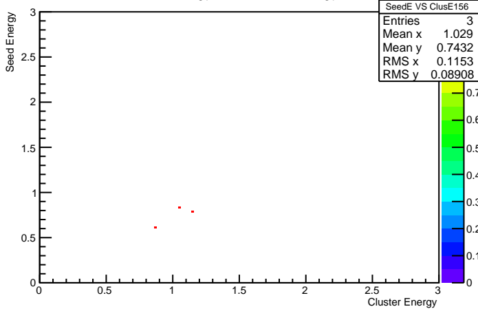
Cluster Energy VS Seed Energy 156
