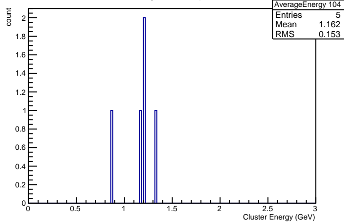
Cluster Energies in Crystal nr 104
