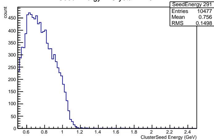
Seed Energy in Crystal nr 291
