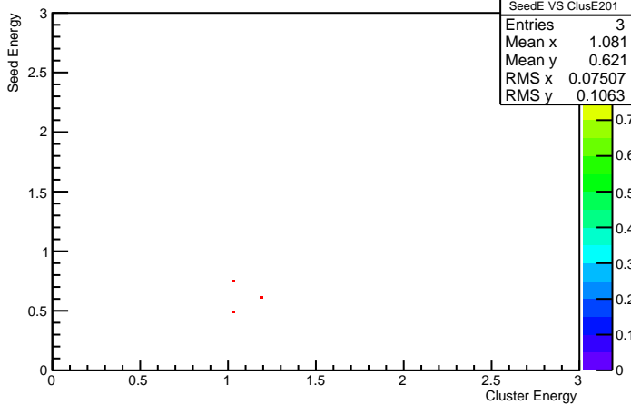
Cluster Energy VS Seed Energy 201
