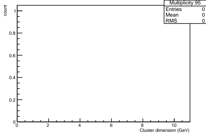
Cluster Dimensions in crystal nr 95
