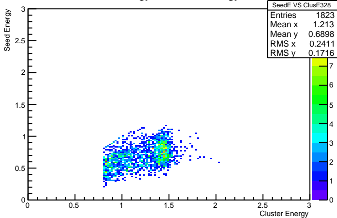
Cluster Energy VS Seed Energy 328
