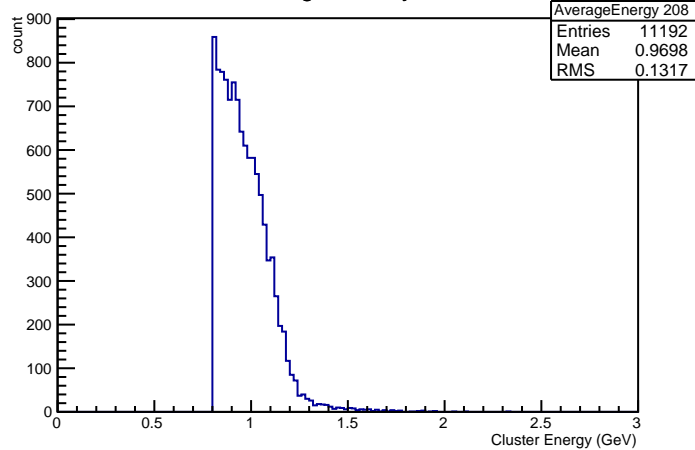
Cluster Energies in Crystal nr 208
