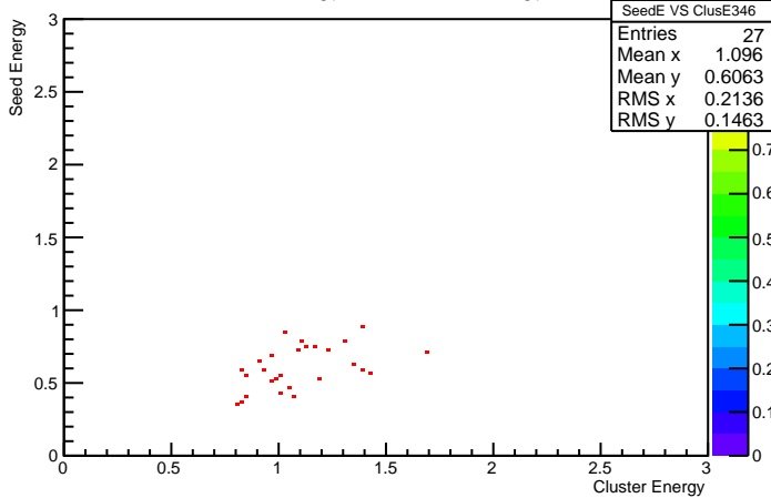
Cluster Energy VS Seed Energy 346
