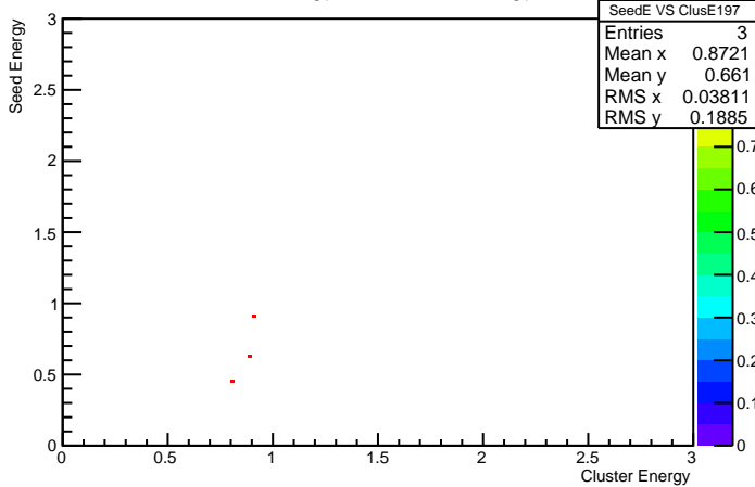
Cluster Energy VS Seed Energy 197
