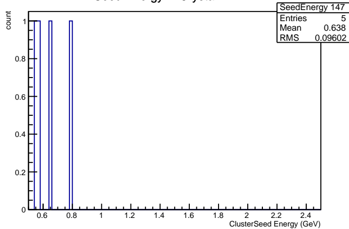
Seed Energy in Crystal nr 147
