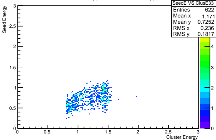
Cluster Energy VS Seed Energy 33
