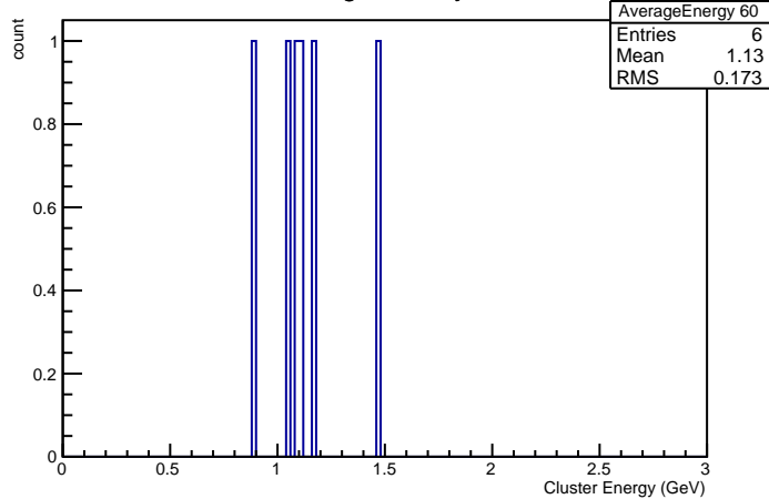
Cluster Energies in Crystal nr 60
