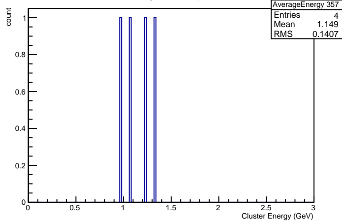
Cluster Energies in Crystal nr 357
