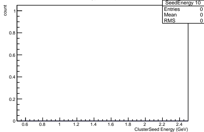
Seed Energy in Crystal nr 10
