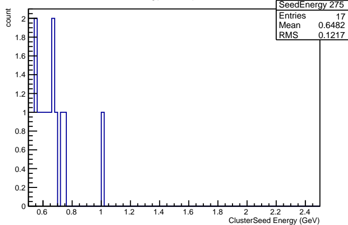
Seed Energy in Crystal nr 275
