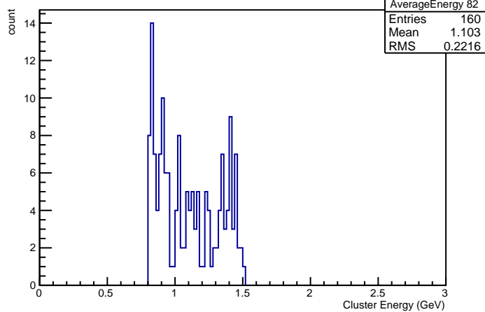
Cluster Energies in Crystal nr 82
