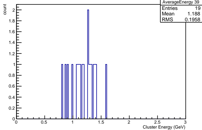
Cluster Energies in Crystal nr 39
