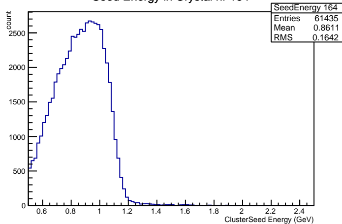
Seed Energy in Crystal nr 164
