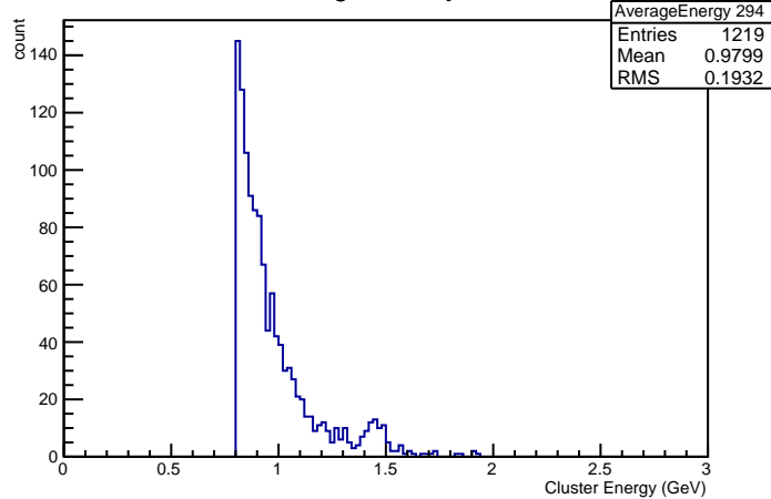
Cluster Energies in Crystal nr 294
