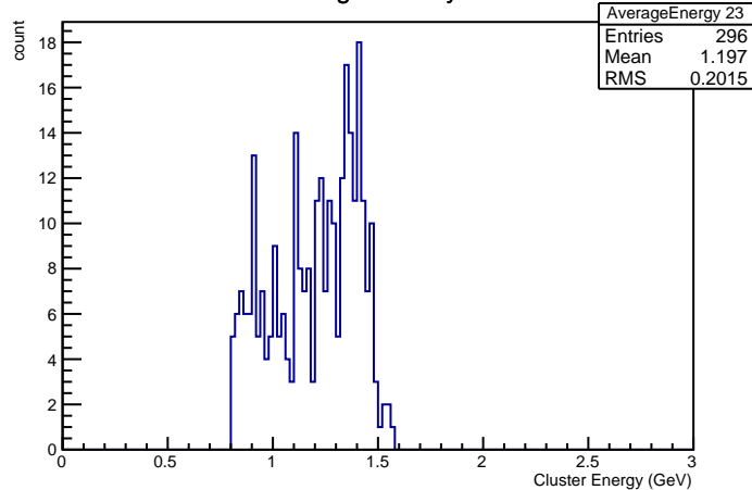
Cluster Energies in Crystal nr 23
