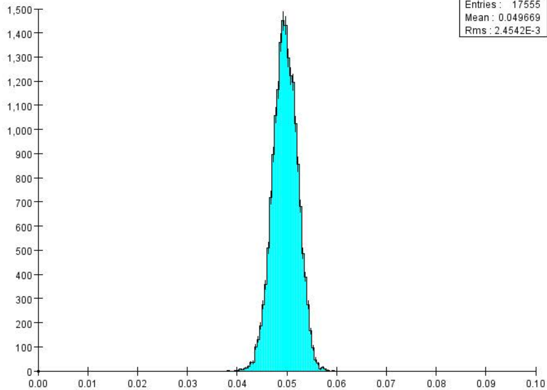
Moller Invariant Mass Unconstrained v31
