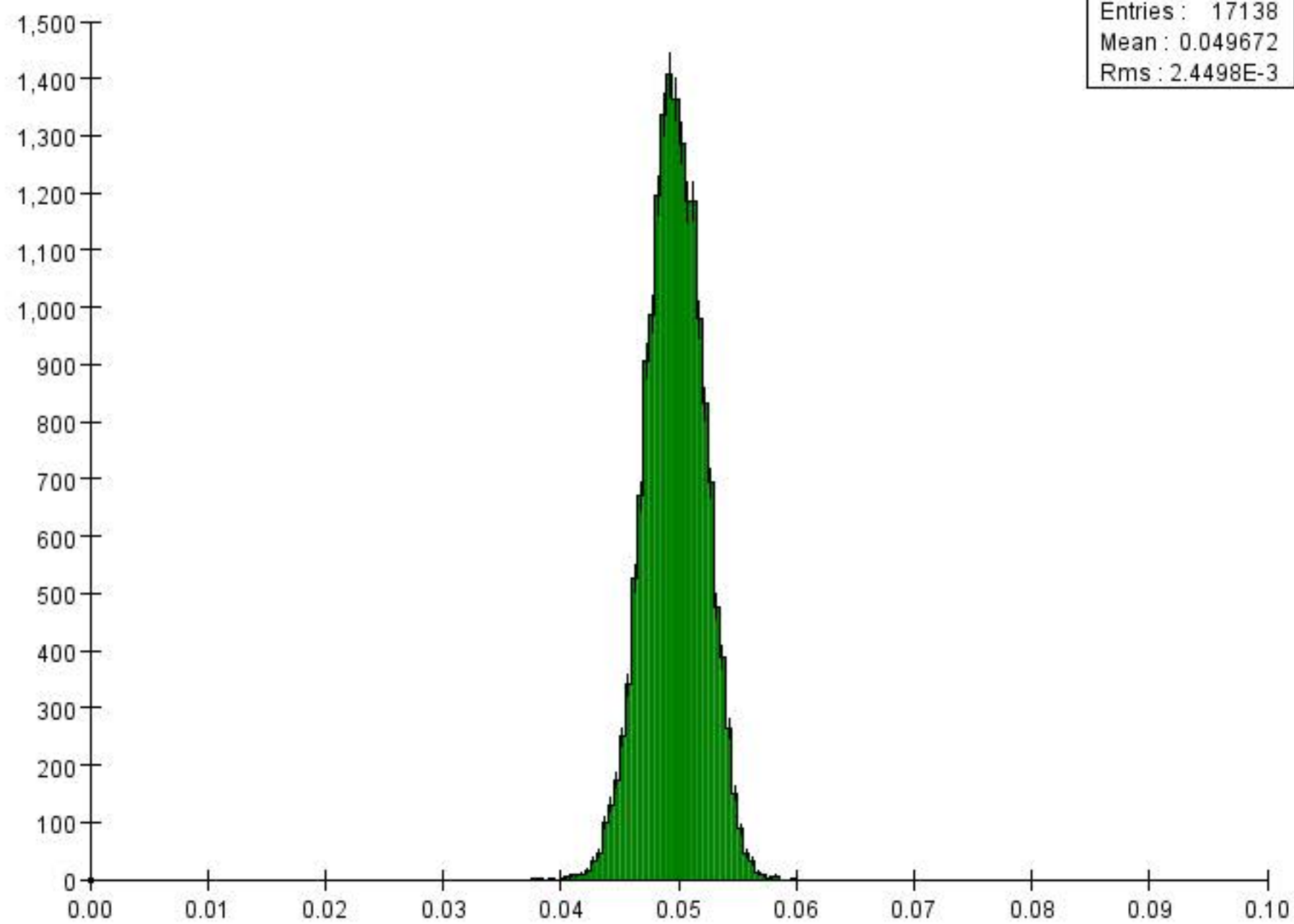
Moller Invariant Mass Unconstrained v20
