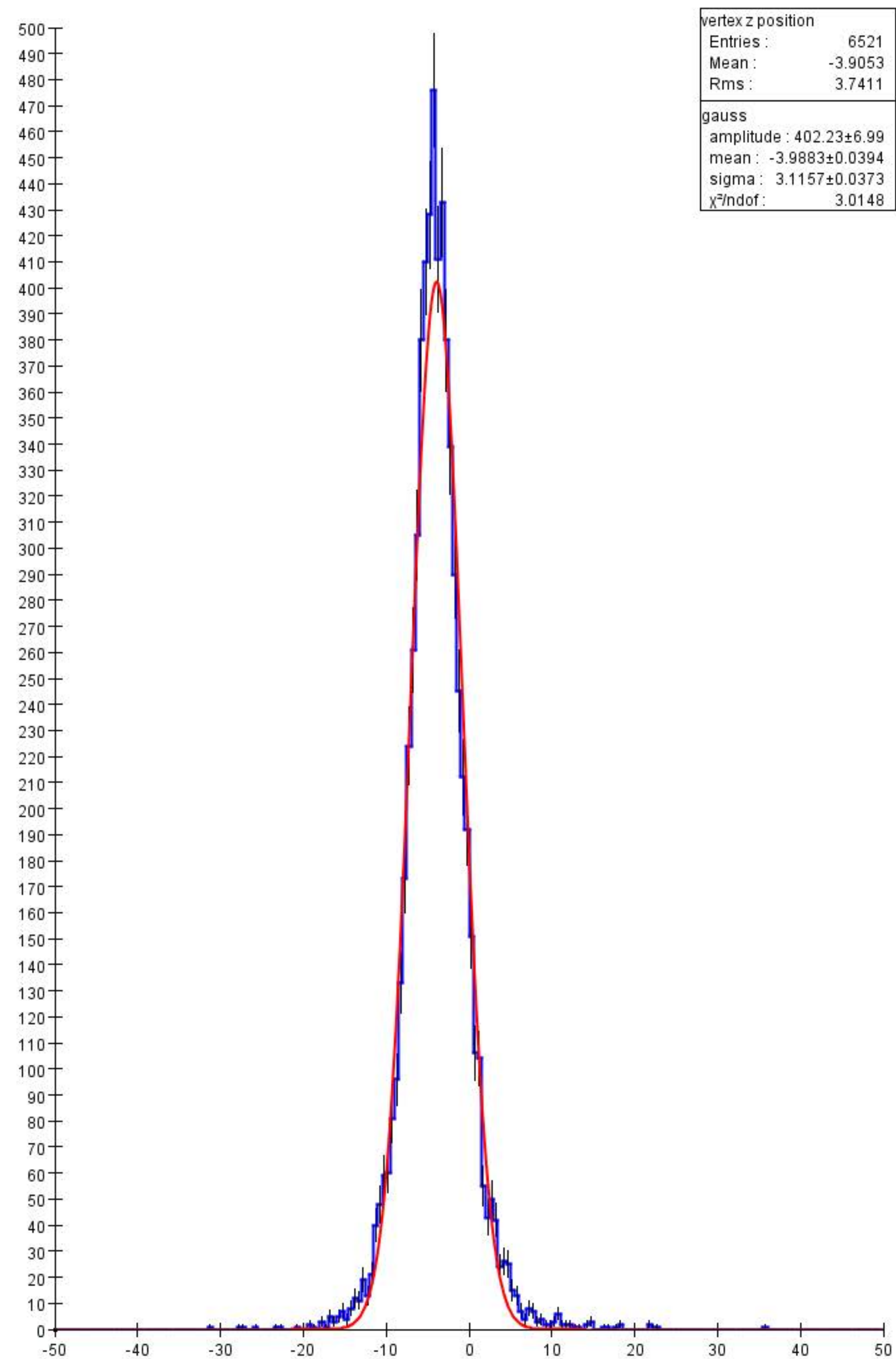
V0 Vertex Z Position #31
