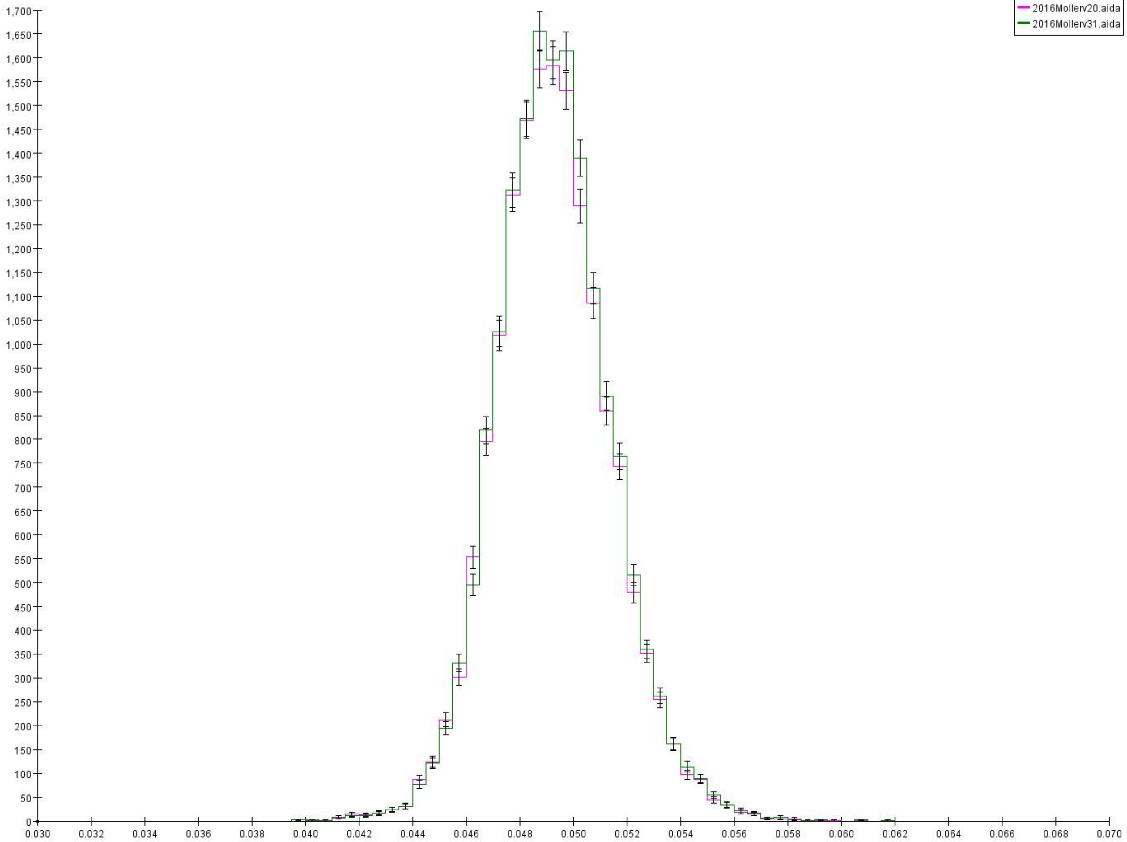
TargetConstrainedMollerVertices - Moller Invariant Mass
