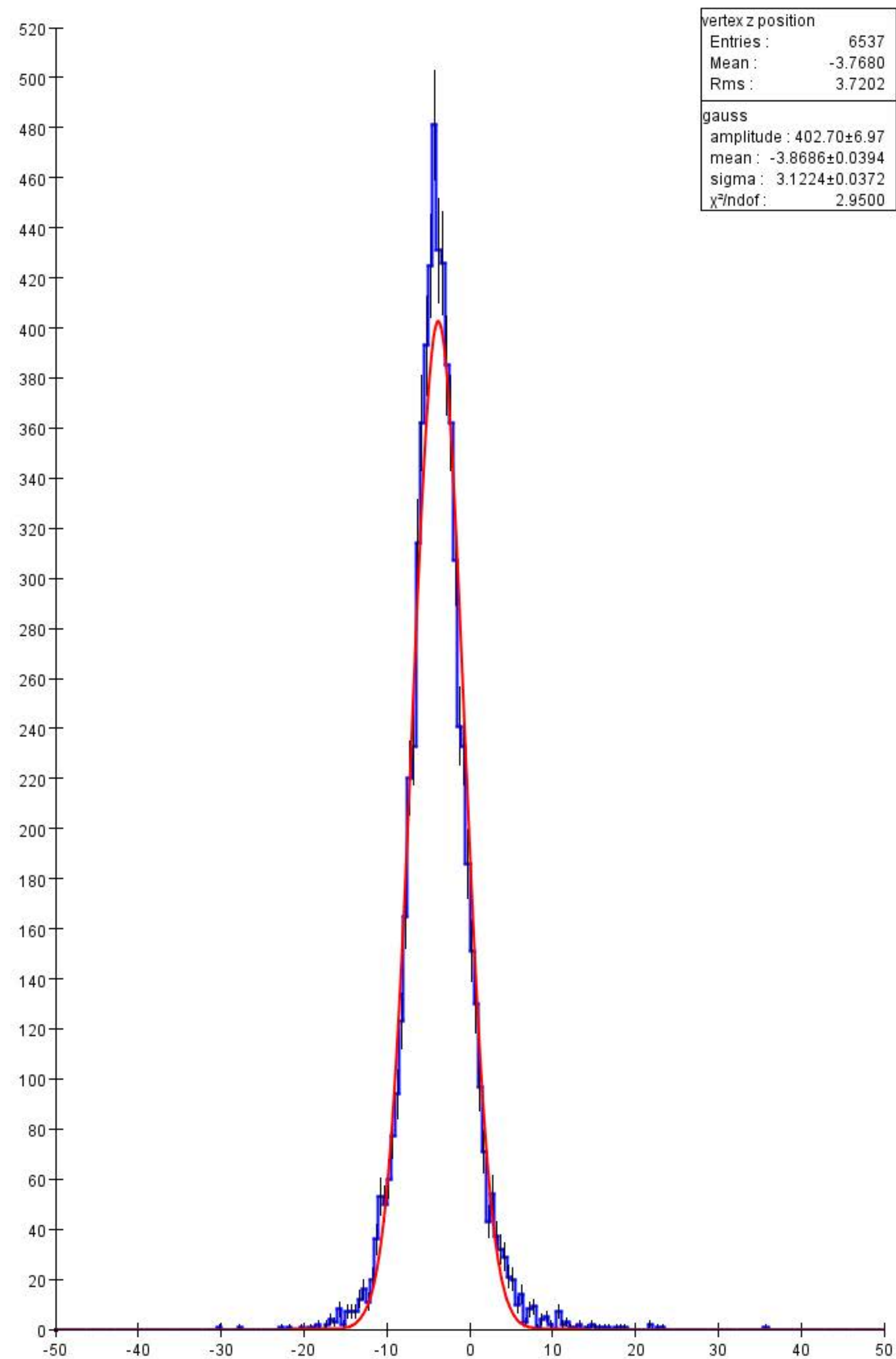
V0 Vertex Z Position #20
