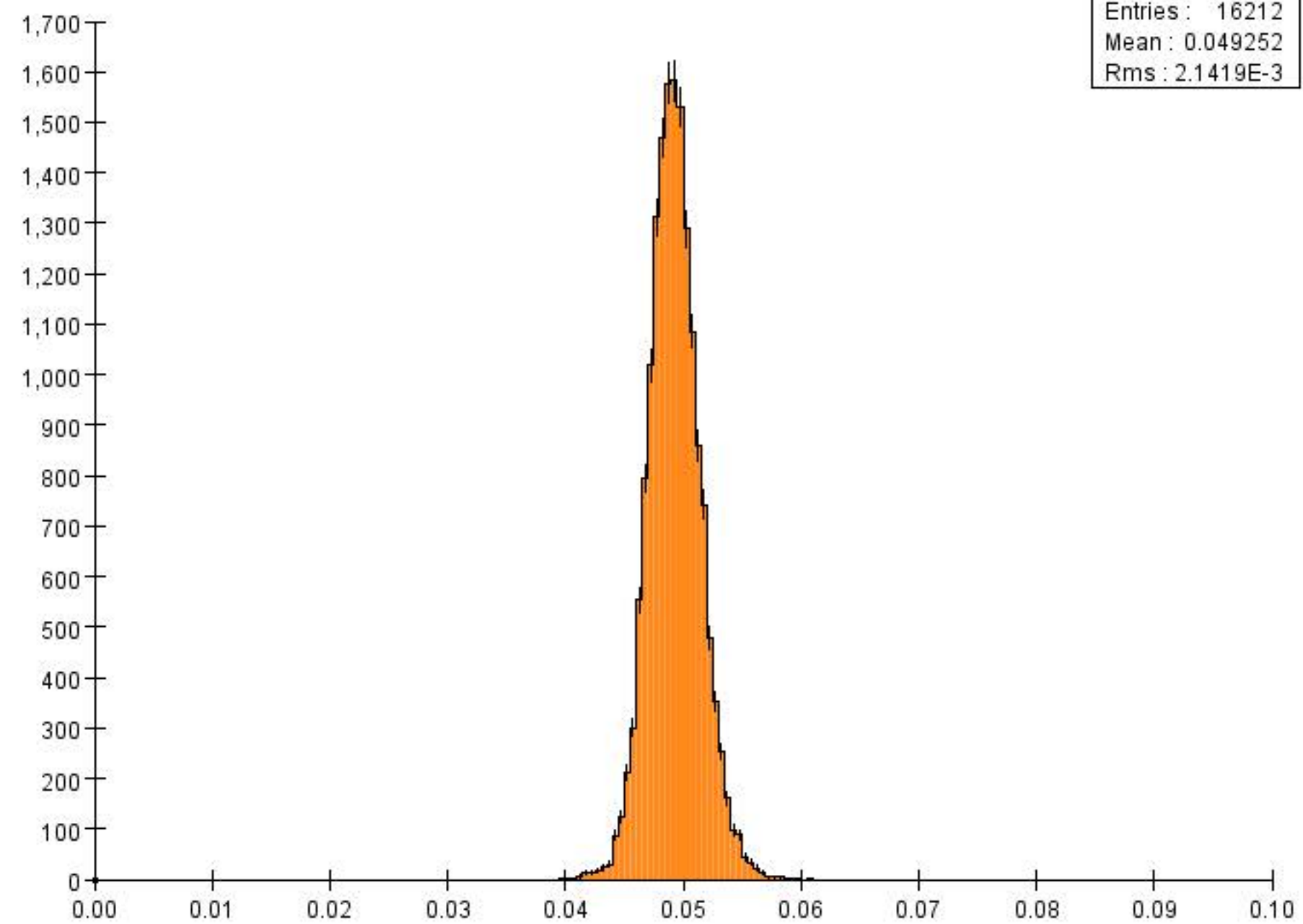
Moller Invariant Mass Target Constrained v20
