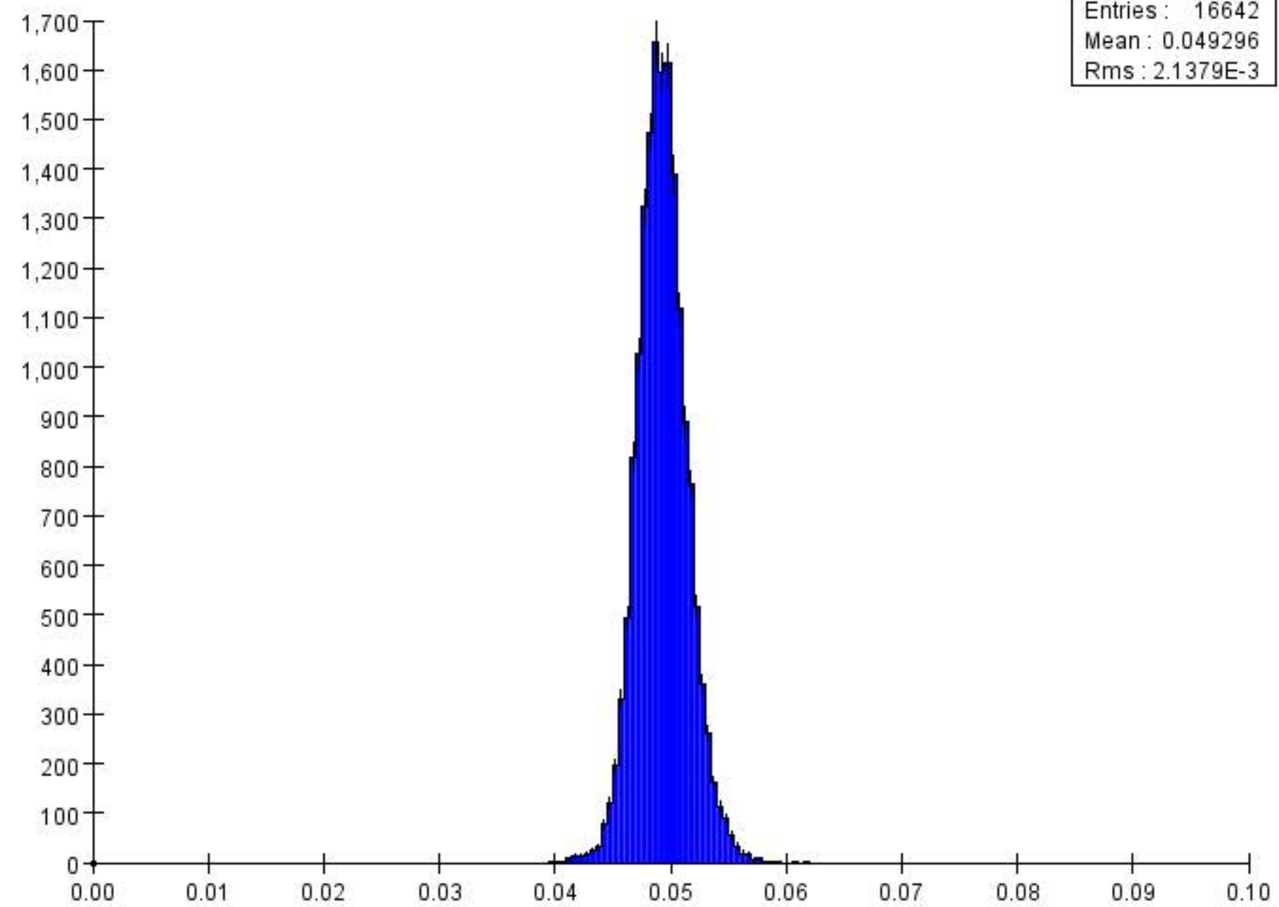
Moller Invariant Mass Target Constrained v31
